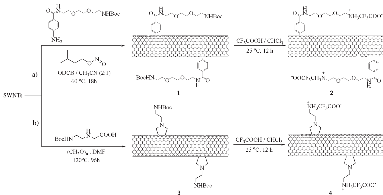
Scheme 1. Functionalization of SWCNTs by a) diazonium salts and b) azomethine ylides, both generated in situ. Boc = tert -butyloxycarbonyl, ODCB = 1,2-dichlorobenzene.
