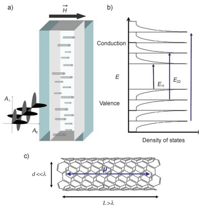
Figure 1. Orientation of nanotubes using a weak magnetic field. a) Nanotubes align parallel to the magnetic field ( H = 0.1 T), which is at right angles to the incident light. The two planes of polarized light A_{\perp} and A_{\parallel} used to obtain the linear dichroism spectra are also shown. b) The electronic spectroscopy of carbon nanotubes are characterized by transitions between the van Hove singularities in the density of states, for example, E_{11} . These unique spectroscopic properties arise from the enormous aspect ratio (c), which approaches the behavior of a one-dimensional solid.
